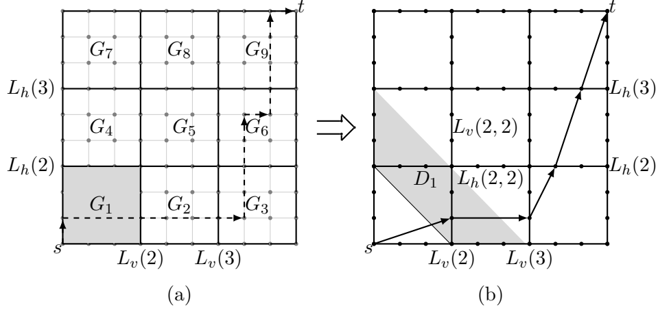
Figure 1: (a) An example of layered grid graph G and its decomposition into blocks (b) Corresponding auxiliary graph H
