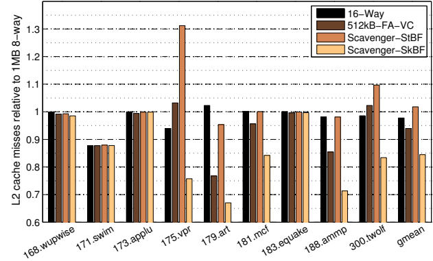
Figure 12. Normalized L2 cache misses for memory-bound applications.
